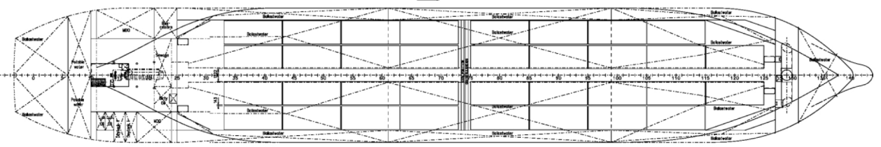
Tanktop
